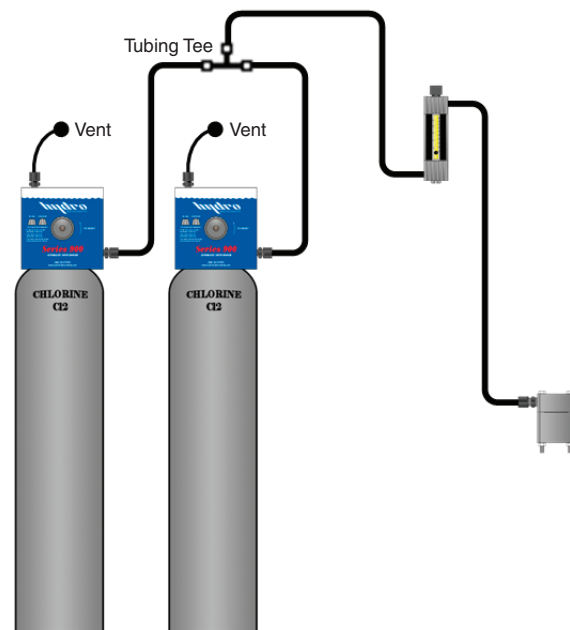
Hydro Instruments Series 900 Gas Chlorination System with Integral Switchover
